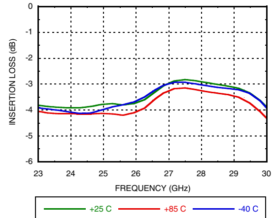
Insertion Loss RFIN to RF3 vs. Temperature
